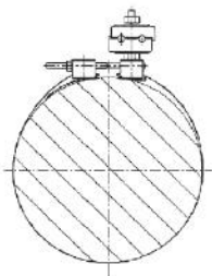
Down Lead Clamp for rubber type pole
